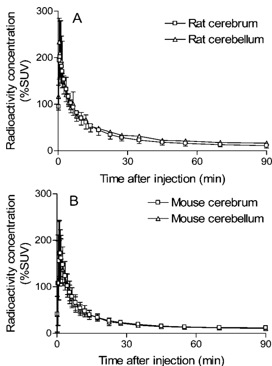
Figure 3. Time course of radioactivity (% SUV) in cerebrum and cerebellum after administration of NCA [ ^{11}\text{C} ]7 to normal rats ( n = 4 ) (A) and normal mice ( n = 4 ) (B). Unilateral error bars indicate the magnitude of SD.
