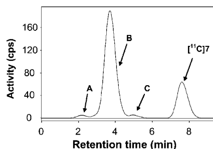
Figure 5. Radiochromatogram of a rat brain extract at 2.83 min after injection of NCA [ ^{11}\text{C} ]7.
