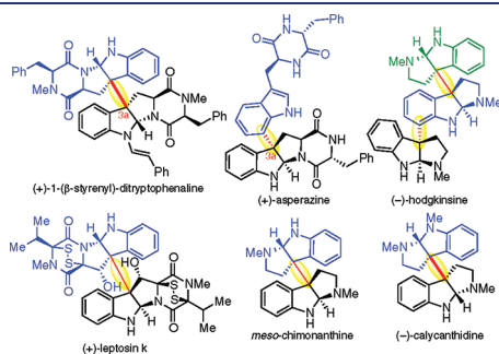
Figure 1. Representative heterodimeric cyclotryptamine alkaloids.
