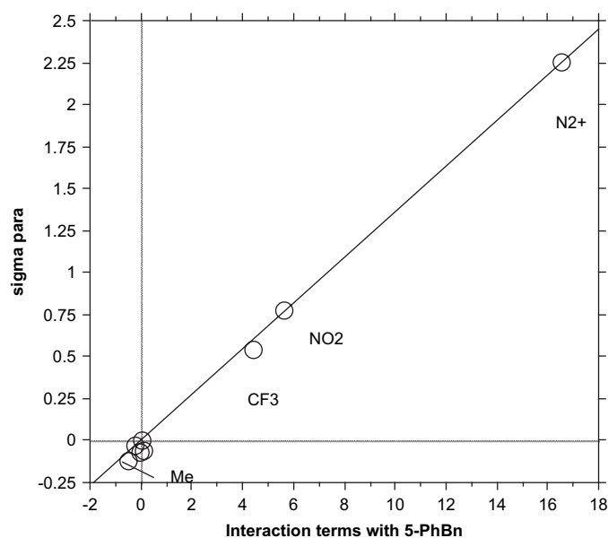
Figure 3. The line corresponds to \sigma_p = (0.136 \pm 0.003) interaction term, n=8 , r^2=0.997 (the reciprocal equation is interaction term = (7.34 \pm 0.14) \sigma_p , n=8 , r^2=0.997 ).
