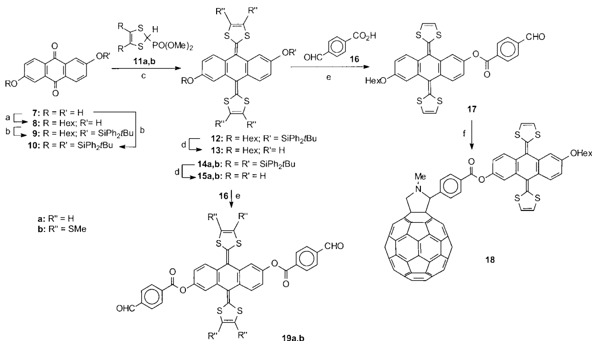
Scheme 1. a) Hexylbromide, K_2CO_3 , DMF; b) tBuPh_2SiCl , imidazole, DMF; c) nBuLi , THF, -78^\circ C ; d) nBu_4NF , THF; e) 4-carboxybenzaldehyde ( 16 ), DCC, DMAP, CH_2Cl_2 ; f) C_{60} , sarcosine, toluene, \Delta .
