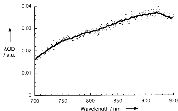
Figure 7. Differential absorption spectra obtained upon picosecond flash photolysis (355 nm) of \approx 1.0 \times 10^{-5} M solutions of triad 25 in nitrogen-saturated benzonitrile with a time delay of 50 ps.
