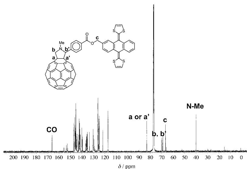
Figure 1. ^{13}\text{C} NMR spectrum for dyad 23 in \text{CDCl}_3 .
