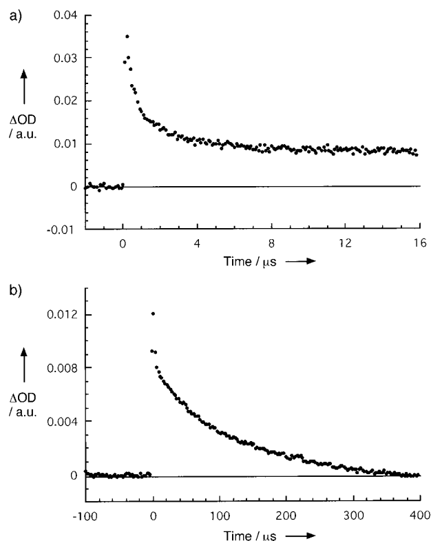
Figure 8. Time-absorption profiles at 1000 nm monitoring the fullerene radical anion decay dynamics of a) C_{60}^{\bullet-}(\text{exTTF})_1^{\bullet+}-(\text{exTTF})_2 and b) C_{60}^{\bullet-}(\text{exTTF})_1-(\text{exTTF})_2^{\bullet+} in triad 25 in nitrogen-saturated DMF.
