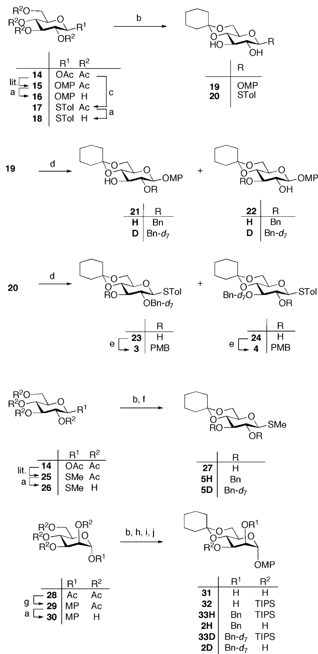
Scheme 3. Reagents and conditions: (a) NaOMe, MeOH, quant. (b) 1,1-dimethoxycyclohexane, CSA, or TsOH·H 2 O, 90% ( 19 ), 71% ( 20 ), 77% ( 27 ), 60% ( 31 ). (c) TolSH, BF 3 ·OEt 2 , 91%, \beta . (d) Ag 2 O (1.5 equiv), BnBr or Bn- d 7 Br (1.1 equiv), KI (0.2 equiv), CH 2 Cl 2 /DMF (10:1), rt, 24 h, 47% ( 21H /22H=2.92:1), 66% ( 21D /22D=1.88:1), 60% ( 23 /24=2.0:1). (e) NaH, PMBCl (1.2 equiv), DMF, 96% ( 3 ), 88% ( 4 ). (f) NaH, BnBr or Bn- d 7 Br (2.2 equiv), DMF, 99% ( 5H ), 70% ( 5D ). (g) MPOH, TMSOTf, 75%. (h) TIPSCl, imidazole, DMF, 95%. (i) NaH, BnBr, or Bn- d 7 Br. (j) TBAF, 97% in two steps ( 2H ), 86% in two steps ( 2D ).
