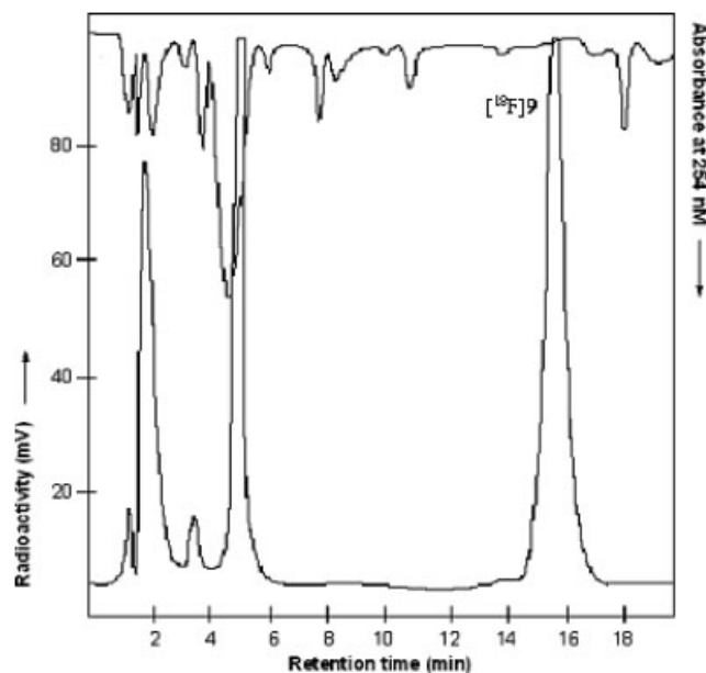
Figure 6. Chromatogram from the HPLC separation of [^{18}\text{F}] PipISB ( [^{18}\text{F}] 9) (upper trace shows absorbance response and lower trace radioactivity response).
