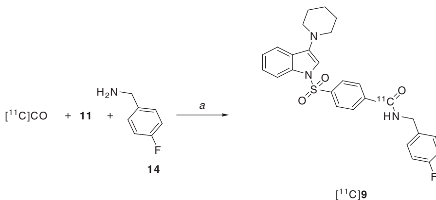
Figure 3. Radiosynthesis of [ ^{11}\text{C} ]PipISB ([ ^{11}\text{C} ]9). Conditions and isolated decay-corrected radiochemical yield; a) \text{Pd}(\text{PPh}_3)_4 , THF, 6000 psi, 150 °C, 5 min, 3.1–11.6% RCY.
