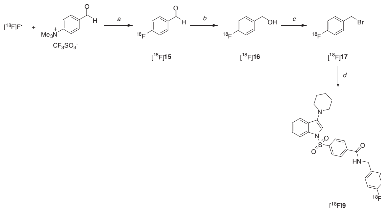
Figure 5. Radiosynthesis of [^{18}\text{F}] PipISB ( [^{18}\text{F}] 9). Conditions and yields: a) Kryptofix 2.2.2, \text{K}_2\text{CO}_3 , DMSO, 110^\circ\text{C} , 7 min; b) aq. \text{NaBH}_4 , RT, 5 min; c) \text{PPh}_3\text{Br}_2 , RT, 5 min; d) \text{NaH} , DMF-DCM, RT, 3 min, 1.5–5.6% RCY (from [^{18}\text{F}] fluoride ion).
