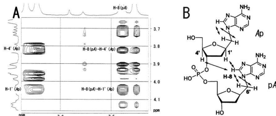
Figure 3. NMR (NOESY) analysis of dA_2 . (A) Contour plot of part of the NOESY spectrum. (B) Schematic of the dimer showing the observed interresidue and intraresidue proton proximity relationships.
