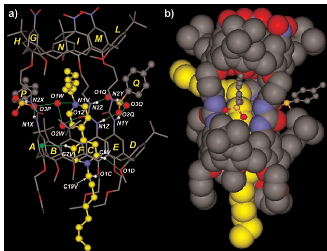
Figure 4. X-ray structure of the complex [11\supset\text{DOV}](\text{TsO})_2 (the \text{DOV}^{2+} component is yellow). a) Partial stick view; b) partial space-filling view. Only the hydrogen atoms involved in weak, attractive intermolecular interactions are shown. The hydrogen bonds and \text{CH}-\pi interactions are denoted by green lines.
