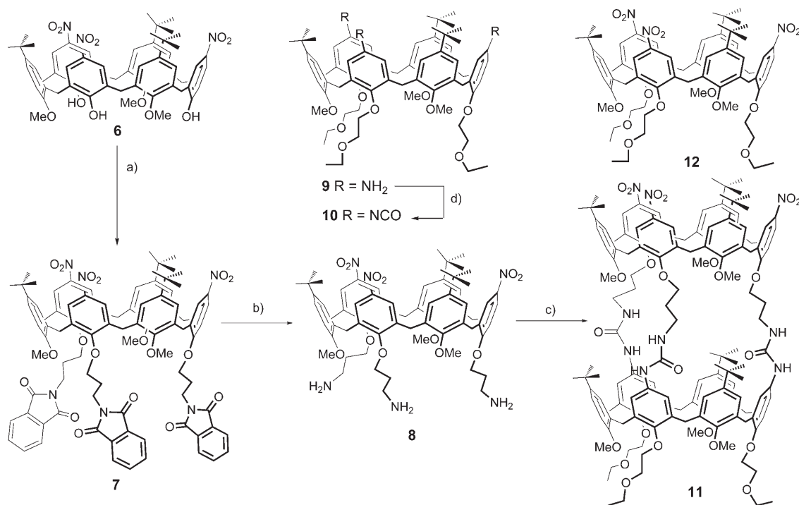
Scheme 2. Reactions and conditions for the synthesis of the double calix[6]arene 11 : a) K 2 CO 3 , 3-( N -bromopropyl)phthalimide, CH 3 CN, reflux, 15 days (30 %); b) NH 2 NH 2 ·H 2 O, EtOH, reflux, 12 h (90 %); c) 10 , CH 2 Cl 2 , 3 h (30 %); d) triphosgene, toluene, reflux, 3 h (70 %).
