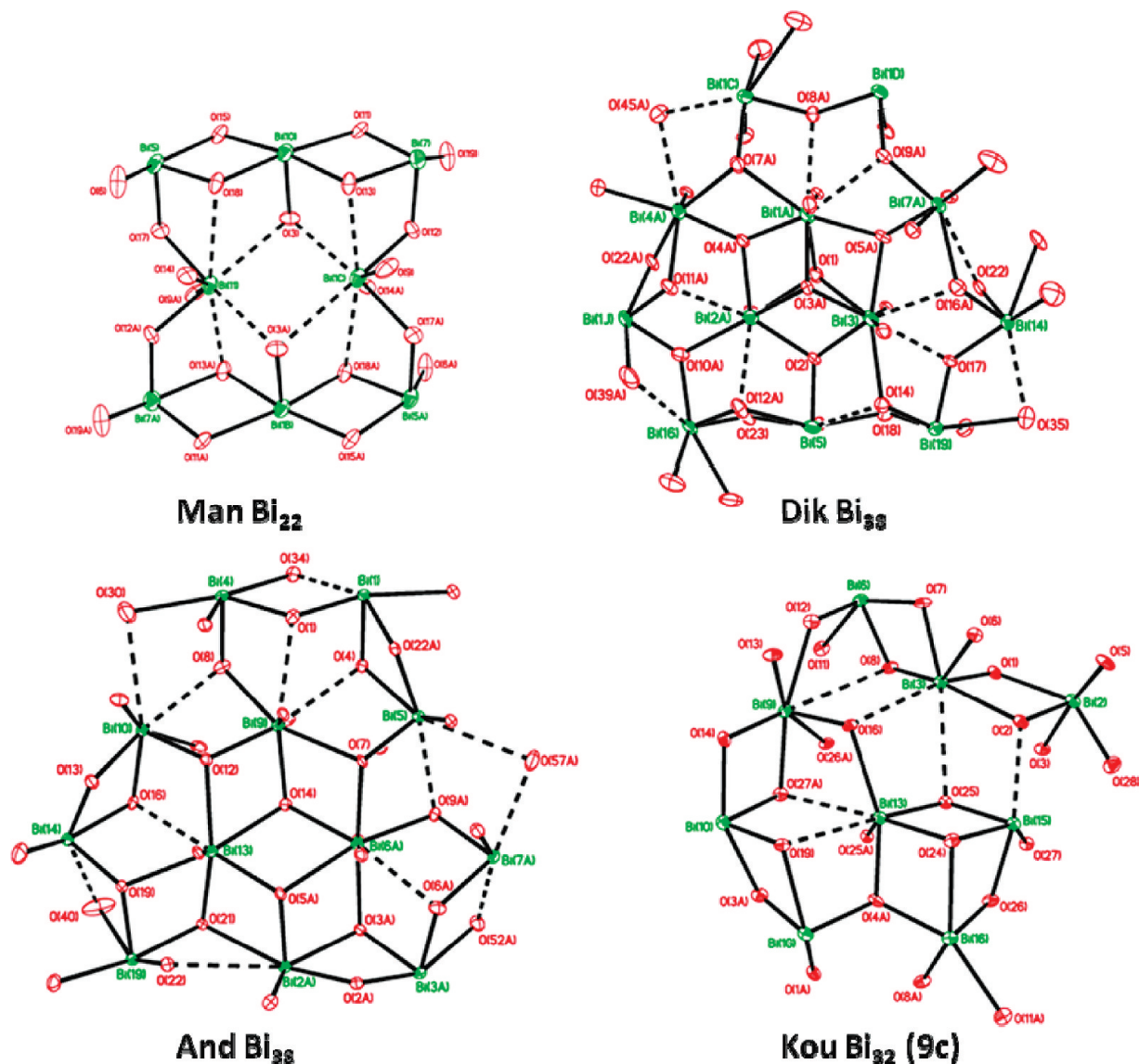
Figure 6. B layers for clusters [\text{Bi}_{22}\text{O}_{26}(\text{OSiMe}_2\text{tBu})_{14}] , 60 [\text{Bi}_{38}\text{O}_{45}(\text{hfac})_{24}] , 57 [\text{Bi}_{38}\text{O}_{44}(\text{Hsal})_{26}(\text{Me}_2\text{CO})_{16}(\text{H}_2\text{O})_2] \cdot 4\text{Me}_2\text{CO} , 58 and \text{Bi}_{32}\text{O}_4(\text{OH})_4(\text{O}-2,6\text{-Ph}_2\text{C}_6\text{H}_3)_{12} 9c .
