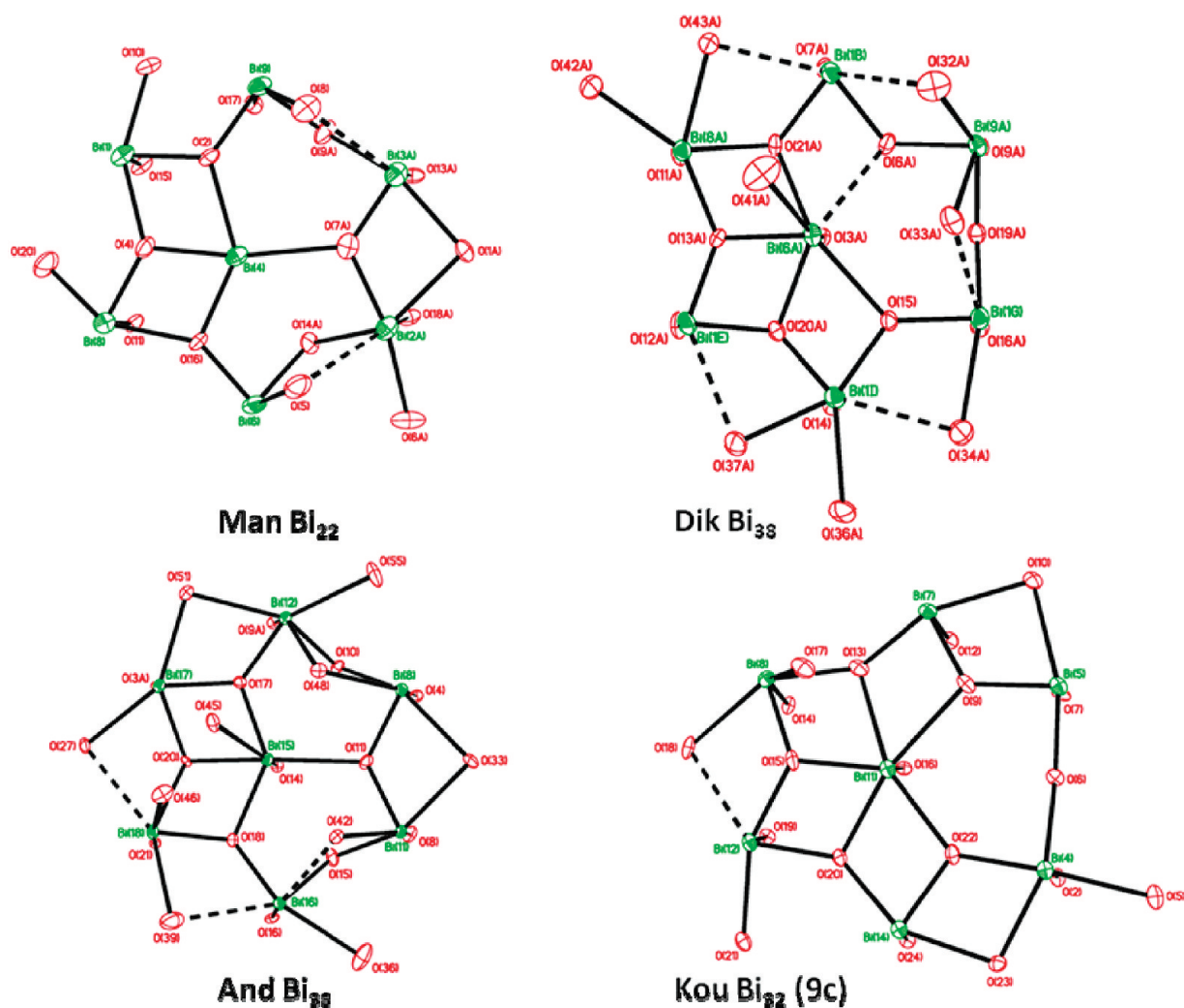
Figure 5. A layers for clusters [\text{Bi}_{22}\text{O}_{26}(\text{OSiMe}_2^t\text{Bu})_{14}] , 60 [\text{Bi}_{38}\text{O}_{45}(\text{hfac})_{24}] , 57 [\text{Bi}_{38}\text{O}_{44}(\text{Hsal})_{26}(\text{Me}_2\text{CO})_{16}(\text{H}_2\text{O})_2] \cdot 4\text{Me}_2\text{CO} , 58 and \text{Bi}_{32}\text{O}_4(\text{OH})_4(\text{O}-2,6\text{-Ph}_2\text{C}_6\text{H}_3)_{12} 9c.
