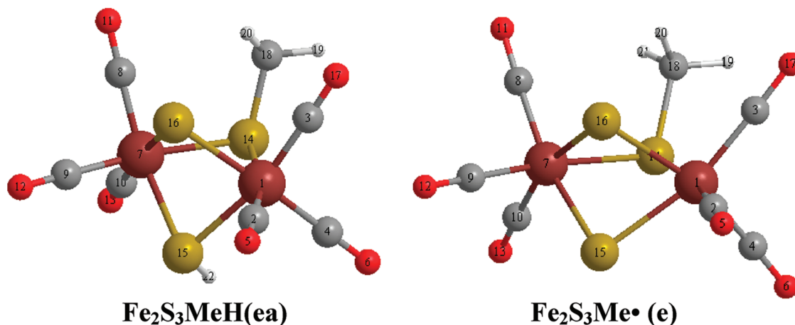
Figure 6. DFT structures of (left) the parent hydrosulfide \text{Fe}_2\text{S}_3\text{MeH}(\text{ea}) and (right) the resulting radical \text{Fe}_2\text{S}_3\text{Me}\cdot(\text{e}) .
