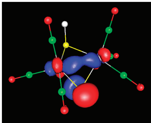
Figure 3. Alpha orbital density of the SOMO of \text{Fe}_2\text{S}_2\text{H}^\bullet . Spin density is primarily located about the two Fe atoms and the bridging S atoms.
