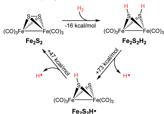
Scheme 6. Thermochemical Cycle for the Addition of Dihydrogen and Subsequent Hydrogen Atom Losses for \text{Fe}_2\text{S}_2 a
