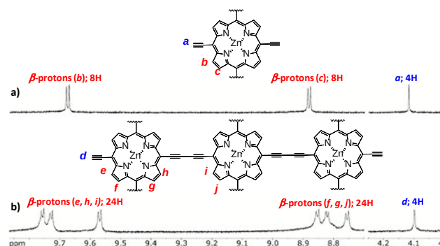
Figure 5. 1 H NMR spectra of a) ZnCP and b) ZnCP 3 in \text{CDCl}_3 (+1% pyridine- d_5 ) at 298 K. Color: \beta -proton signals, red; alkyne proton, blue.
