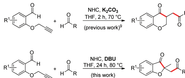
Scheme 1. Cascade Catalysis Using NHC
