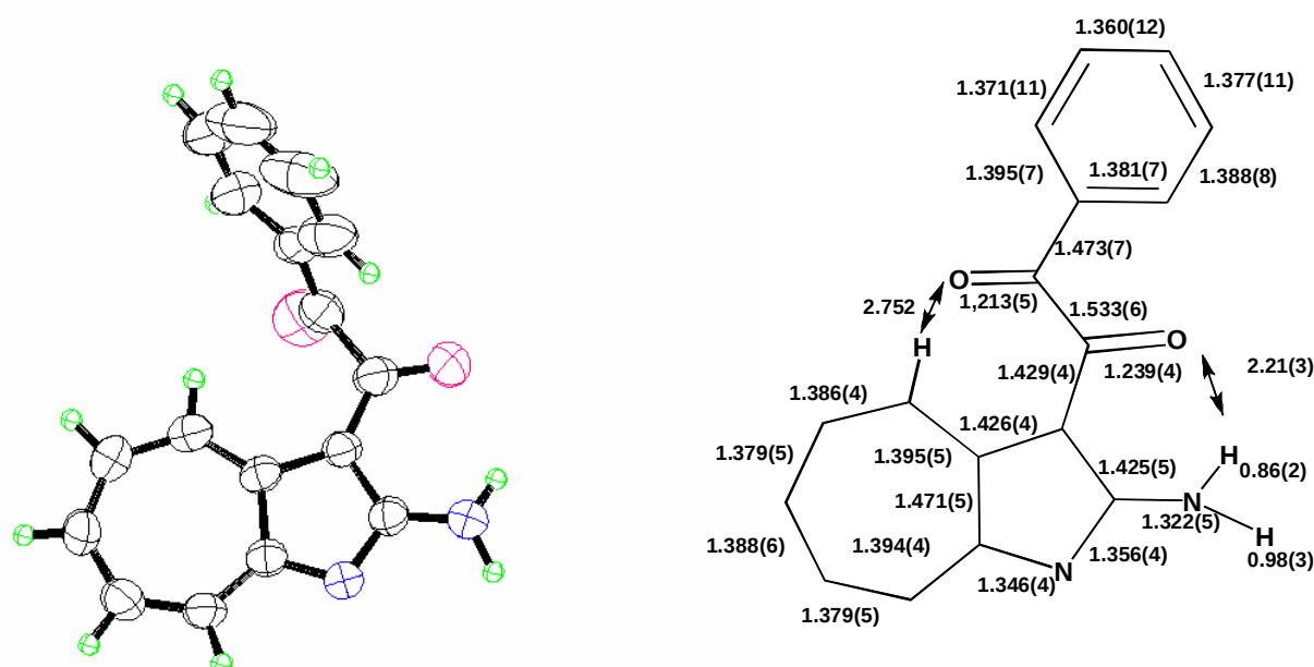
Figure 2. ORTEP drawing with thermal ellipsoids (50% probability) and bond lengths of 13 .
