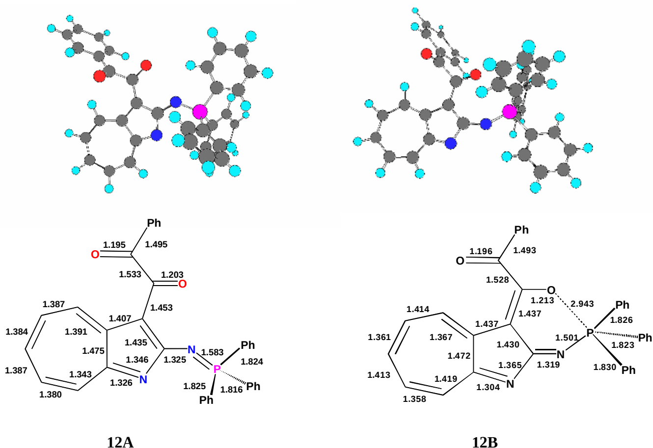
Figure 1. Calculated bond lengths ( \text{\AA} ) and the optimized structures of 12A and 12B .
