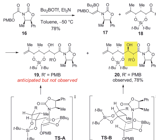
Figure 5. Attempted asymmetric aldol reaction of aldehyde 18 with reagent 16 in the synthesis of cytovaricin.
