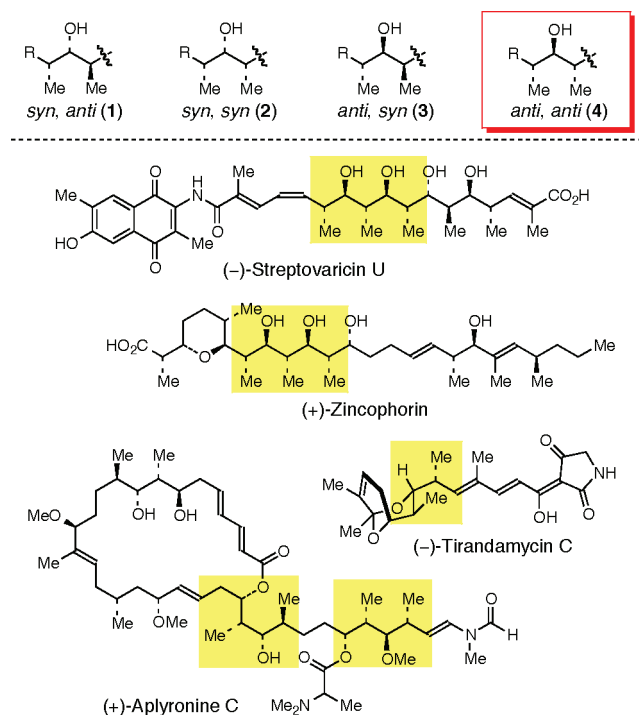
Figure 1. Structure of stereotriads and representative anti,anti -stereotriad containing polyketide natural products.
