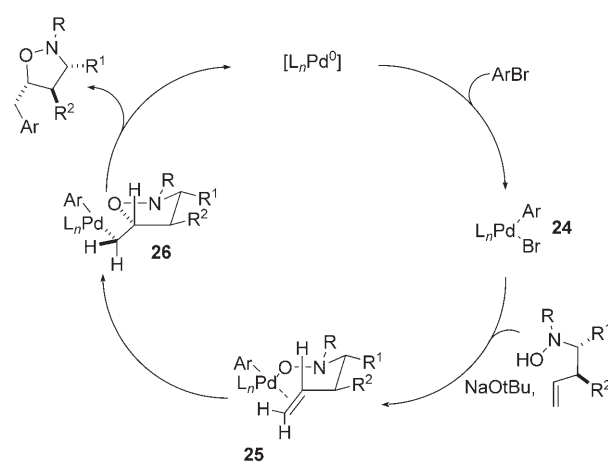
Scheme 1. Catalytic cycle of the Pd-catalyzed carboetherification reaction of N -butenylhydroxylamines.
