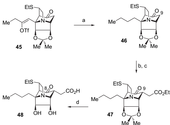
Scheme 11. (a) 1 atm \text{H}_2 , 10% Pd/C, MeOH, 23 °C, 89%; (b) LDA, \text{ICH}_2\text{CO}_2\text{Et} , THF, HMPA, 0 °C; (c) DBU, PhMe, 80 °C, 58% (two steps); (d) 2.5 M \text{HCl} , THF, 60 °C, 96%.
