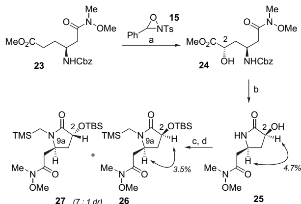
Scheme 6. (a) LHMDS, THF, -78^{\circ}\text{C} , 57%; (b) 1 atm H 2 , 10% Pd/C, MeOH, 23^{\circ}\text{C} , 94%; (c) TBSCl, imidazole, DMF, 23^{\circ}\text{C} , 91%; (d) NaH, TMSCH 2 Cl, DMF, 23^{\circ}\text{C} , 70%.
