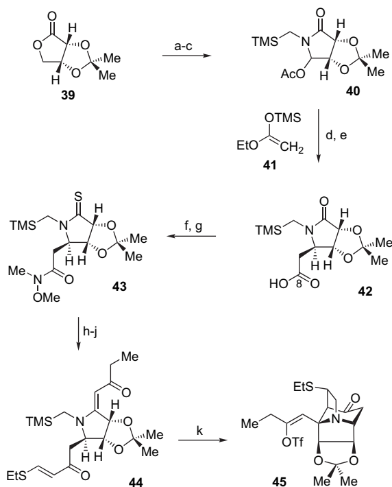
Scheme 10. (a) \text{TMSCH}_2\text{NH}_2\text{Cl} , \text{Et}_3\text{N} , THF, 70 °C, 97%; (b) \text{SO}_3 \cdot \text{Py} , \text{Et}_3\text{N} , DMSO, 23 °C; (c) \text{Ac}_2\text{O} , pyridine, 23 °C, 69% (two steps); (d) \text{TMSOTf} , \text{CH}_2\text{Cl}_2 , 23 °C, 72%; (e) \text{LiOH} , THF, \text{H}_2\text{O} , 23 °C, 96%; (f) Lawesson's reagent, PhMe, 65 °C, 95%; (g) \text{MeONHMe} \cdot \text{HCl} , EDC, \text{Et}_3\text{N} , \text{CH}_2\text{Cl}_2 , 23 °C, 62%; (h) 1-bromo-2-butanone; \text{Ph}_3\text{P} , \text{Et}_3\text{N} , \text{CH}_3\text{CN} , 23 °C, 81%; (i) \text{HCCMgBr} , THF, 23 °C; (j) \text{EtSH} , \text{Et}_3\text{N} , \text{CH}_2\text{Cl}_2 , 23 °C, 58% (two steps); (k) \text{Ti}_2\text{O} , TBAT, \text{CHCl}_3 , –45 to 23 °C, 71%.
