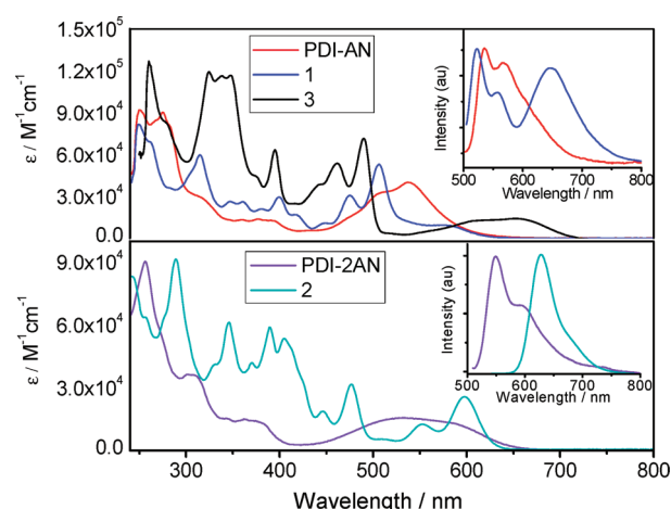
Figure 2. UV–vis absorption and fluorescence emission (inset) spectra of PDI-AN , 1 , 3 , PDI-2AN , and 2 in CH 2 Cl 2 .
