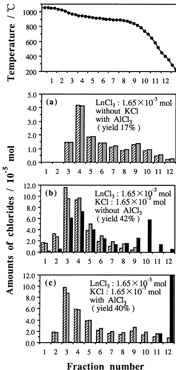
Fig.1. Temperature dependence curve, and lanthanoid and complex former distributions for a mixture of \text{PrCl}_3 and \text{NdCl}_3 . Complex former is \text{AlCl}_3 (a), KCl (b), and KCl- \text{AlCl}_3 (c).
