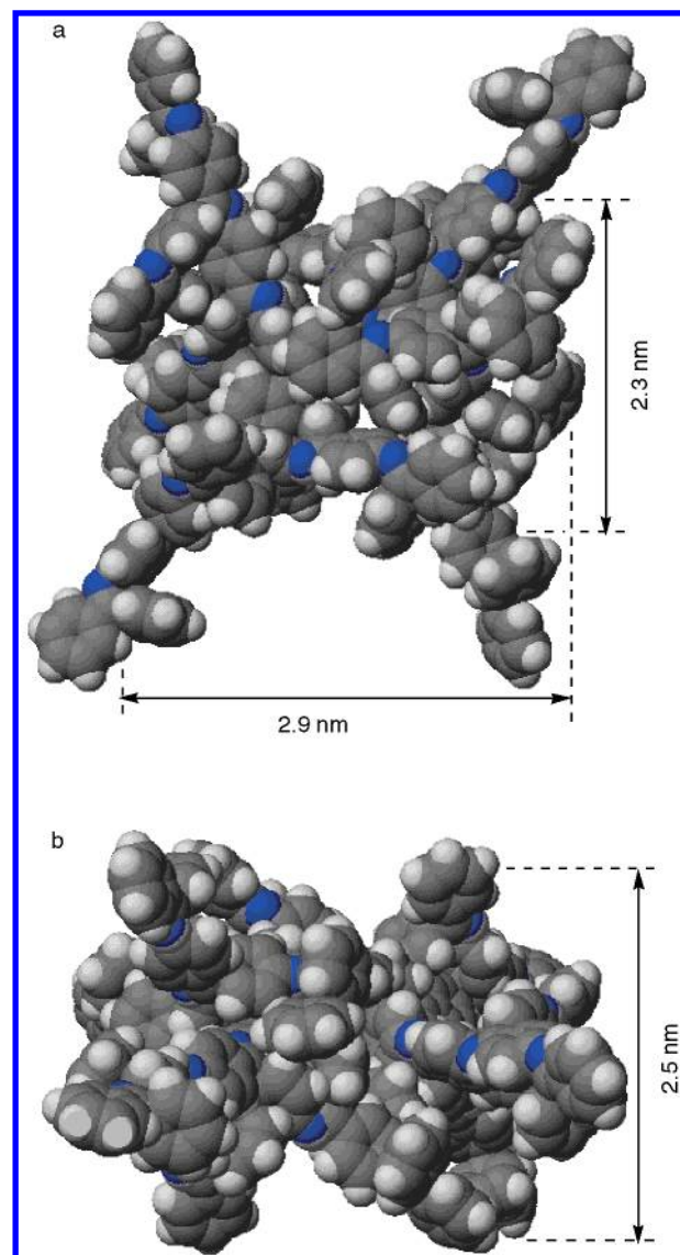
Figure 3. Molecular model of DPA G4 based on the crystal structure of DPA G2.
