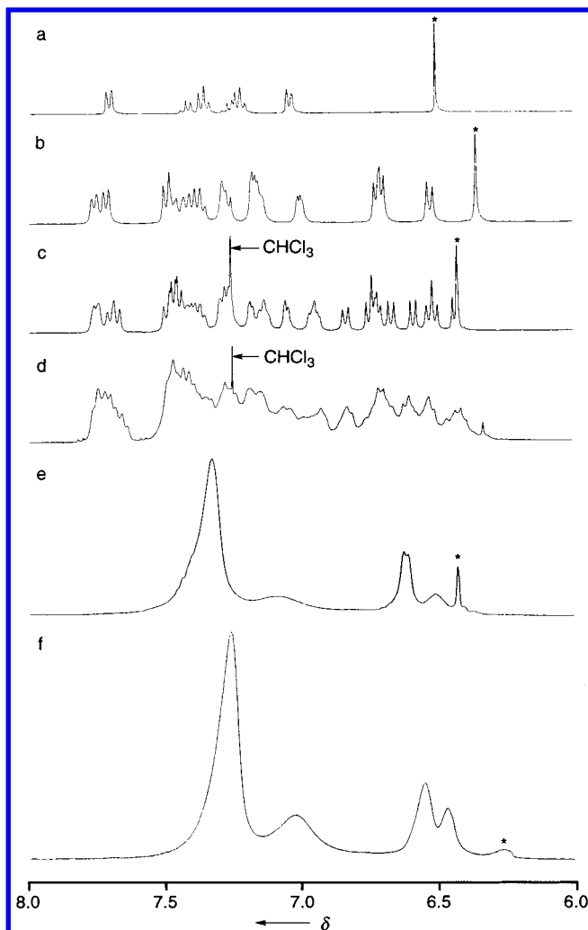
Figure 7. ^1\text{H} NMR spectra of DPAs (a) G1, (b) G2, (c) G3, and (d) G4 in \text{CDCl}_3 at 30 ^\circ\text{C} , and those of DPAs (e) G3 and (f) G4 in \text{DMSO}-d_6 at 130 ^\circ\text{C} . The marked peaks (*) are attributed to the four protons of the phenyl ring in the core of the DPAs.
