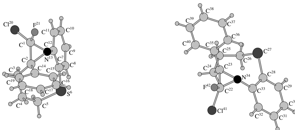
Fig. 2. Structures of two independent molecules of ( RS,RS )-1-chloro-1-fluoro-1a-phenyl-1a,2,3,4-tetrahydro-1 H -azirino[2,1- e ][1,6]-benzothiazocine ( Id ) according to the X-ray diffraction data.
