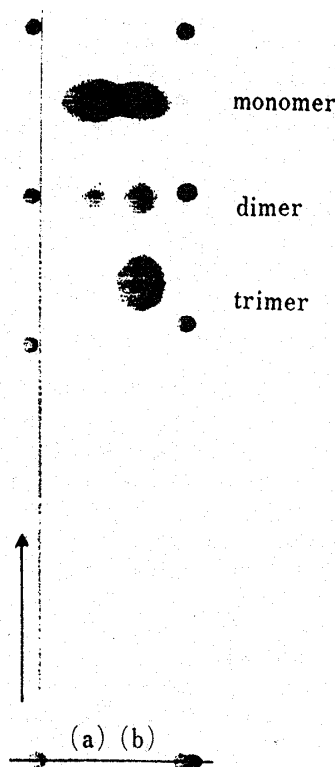
Fig. 4. Homochromatography of Products obtained by Partial Digestion with Venom Phosphodiesterase (a) d^{32}pGGAATTCC and (b) d^{32}pGGaraAATTCC
