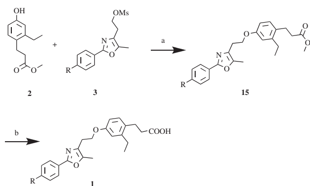
Scheme 1. Reagents and conditions: (a) K 2 CO 3 , MeCN, reflux, 1 d, 70–90%; (b) NaOH, EtOH, r.t., overnight, 85–95%.
