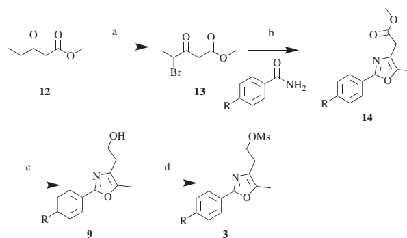
Scheme 3. Reagents and conditions: (a) \text{Br}_2 , \text{CH}_2\text{Cl}_2 , 5^\circ\text{C} , overnight, 98%; (b) 90^\circ\text{C} , 18 h, 65–75%; (c) \text{NaBH}_4 , \text{MeOH} , \text{CH}_2\text{Cl}_2 , 0^\circ\text{C} , 80–95%; (d) \text{MsCl} , \text{Et}_3\text{N} , \text{CH}_2\text{Cl}_2 , 0^\circ\text{C} , 1 h, 95–98%.
