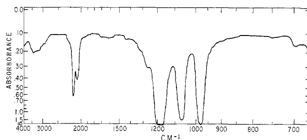
Figure 1.—Infrared spectrum of \text{NaN}_3 \cdot 1.3\text{SO}_2 (KBr pellet).
