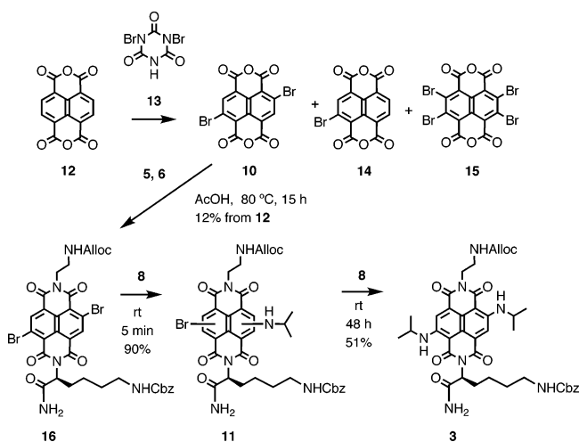
SCHEME 2. Fast, Mild, and Safer Synthesis of N,N -NDI 3 and Synthesis of N,Br -NDI 11
