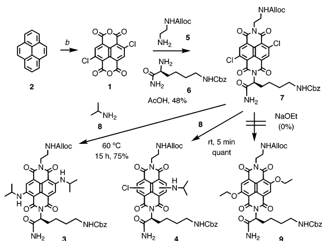
SCHEME 1. Summary of the Previous Synthesis of 3 and 4 2,3,a
