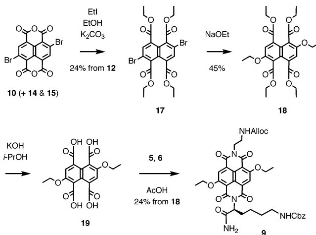
SCHEME 3. Synthesis of O,O -NDI 9
