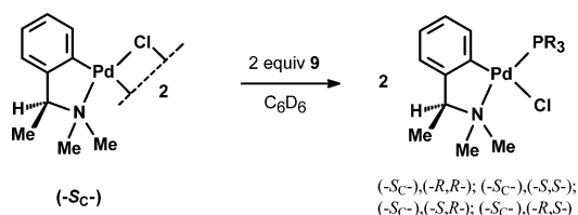
Scheme 4 Reaction of 9 with a chiral Pd-complex.
