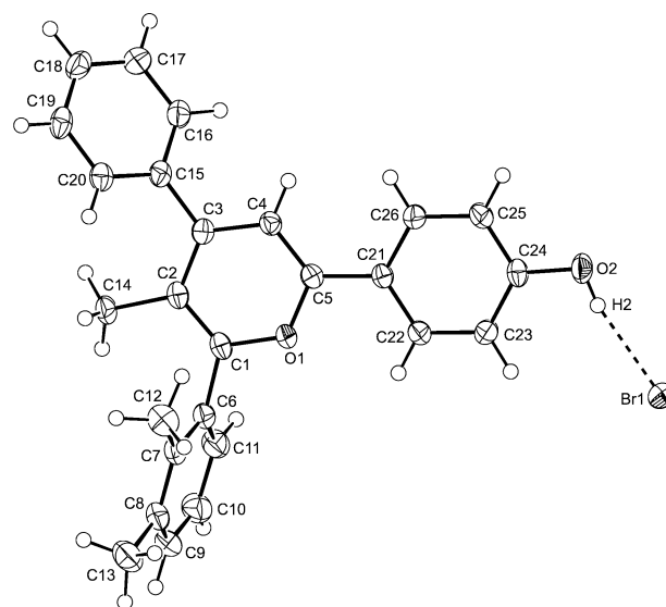
Fig. 2 Molecular structure of 8 in the crystal. Displacement ellipsoids are shown at the 50% probability level. The \text{O--H} \cdots \text{Br} hydrogen bond is drawn with dashed lines. Selected bond lengths ( \text{\AA} ): \text{C1--O1} : 1.358(2), \text{O1--C5} : 1.346(3), \text{C5--C21} : 1.452(3), \text{C1--C6} : 1.484(3), \text{O2} \cdots \text{Br1} : 3.1438(18). Torsion angle ( ^\circ ): \text{C7--C6--C1--C2} : +73.0(3) .
