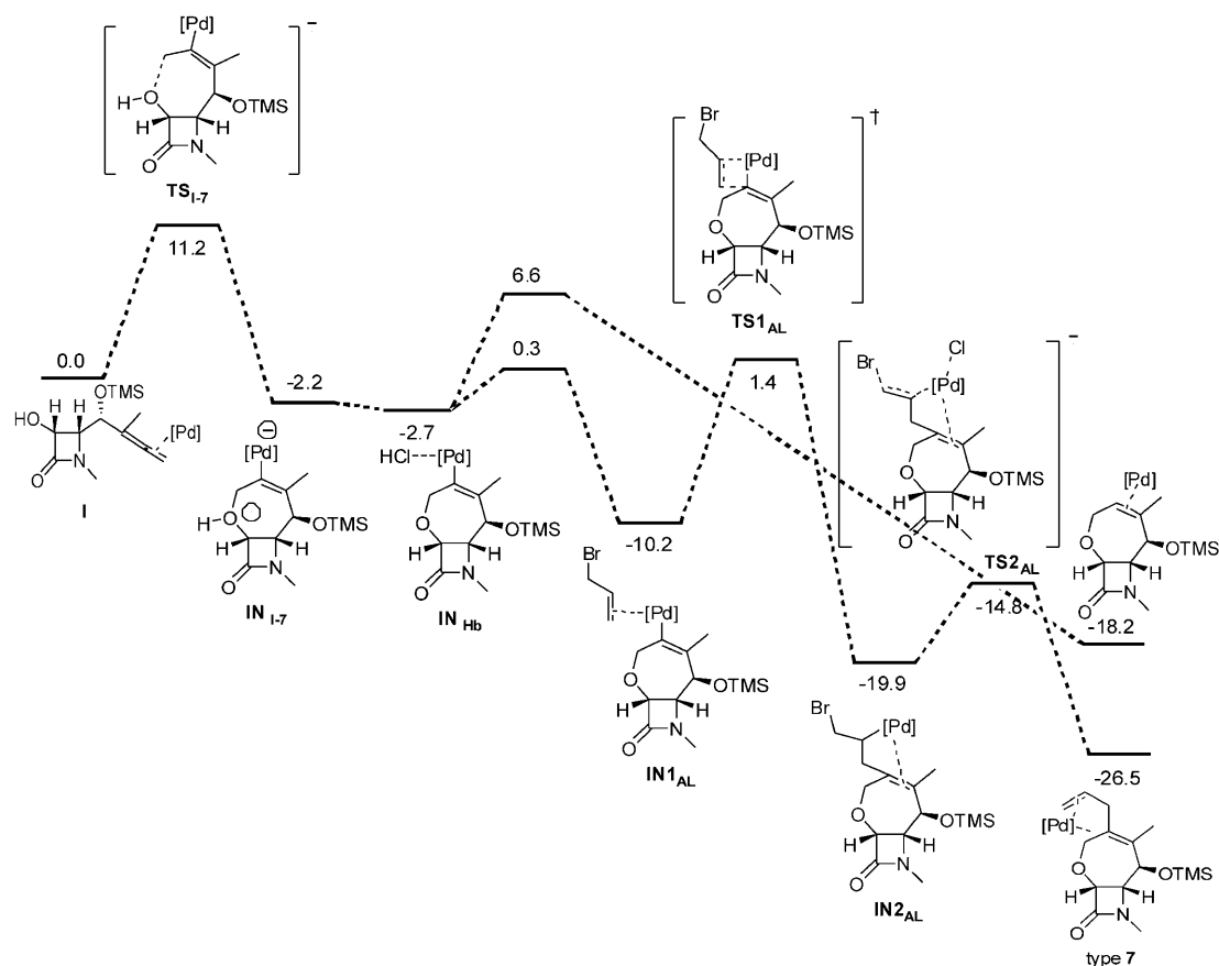
Figure 6. Free energy profile (kcal mol -1 ) for the transformation of \gamma -allenol I into the tetrahydrooxepine of type 7 . Formation of the corresponding bicyclic from protonolysis of the intermediate IN Hb is shown for comparison.
