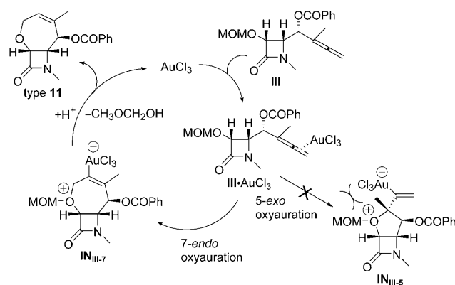
Scheme 4. Mechanistic explanation for the \text{Au}^{\text{III}} -catalyzed heterocyclization of MOM-protected \gamma -allenol derivatives III .
