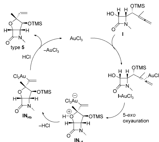
Scheme 2. Mechanistic explanation for the Au III -catalyzed heterocyclization of \gamma -allenol 1 .
