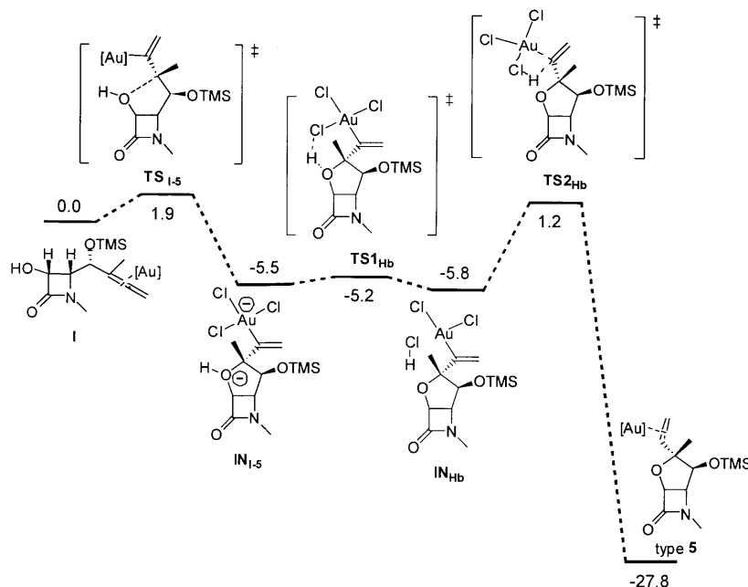
Figure 5. Free energy profile (kcal mol -1 ) for the transformation of \gamma -allenol 1 into the tetrahydrofuran of type 5 .
