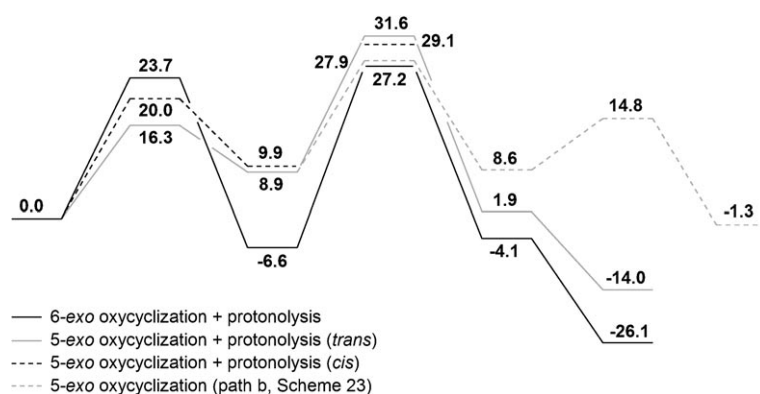
Figure 20. Free energy profile ( \text{kcal mol}^{-1} ) of potential intramolecular hydroalkoxylation/cyclizations of La-alkoxy complex 21 .
