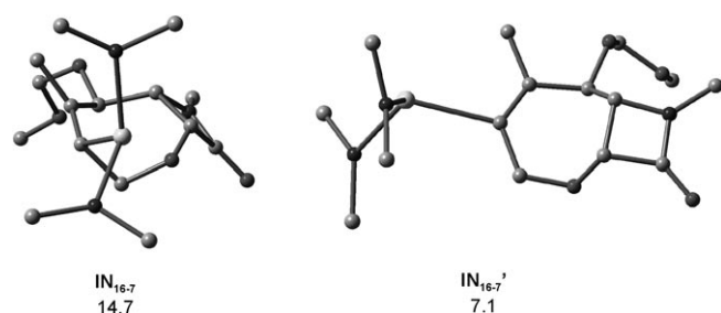
Figure 16. Optimized geometries of 7- endo oxacyclic conformers IN_{16-7} and IN_{16-7'} .
