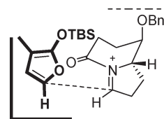
Figure 2. Proposed transition state for the threo -selective VMR of N,O -acetal 8 with 2-methylsilyloxyfuran 9 .
