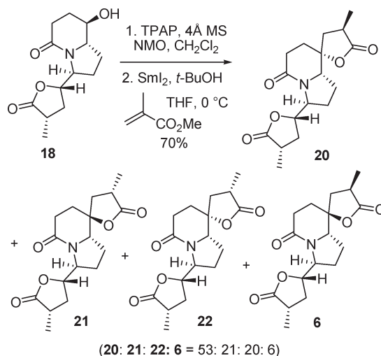
Scheme 5. Final Synthesis of 9- epi and (–)-Sessilifoliolamide J
