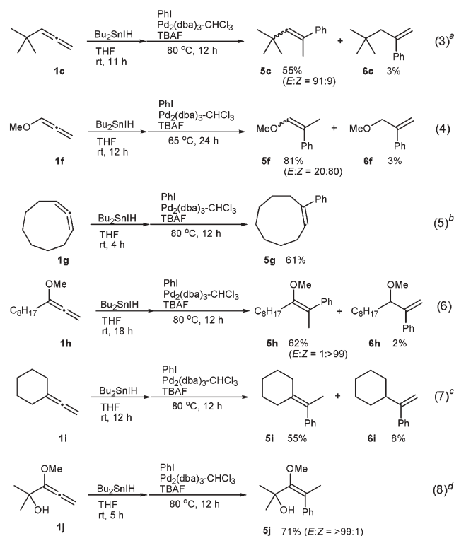
Scheme 4 Hydrostannylation and one-pot coupling reactions. Reagents : THF (1 mL), allene (1 mmol), \text{Bu}_2\text{SnIH} (1 mmol), \text{PhI} (1 mmol), Pd cat. (0.01 mmol), TBAF (1 M solution in THF, 3.0 mmol). a \text{Et}_3\text{B} (0.1 mmol) was added at the hydrostannylation step; \text{PPh}_3 (0.04 mmol) was added at the coupling step. b \text{Bu}_2\text{SnIH} (1.2 mmol) was used; \text{Et}_3\text{B} (0.1 mmol) was added at the hydrostannylation step; \text{PPh}_3 (0.04 mmol) was added at the coupling step. c \text{PPh}_3 (0.07 mmol) was added at the coupling step. d \text{PhI} (1.2 mmol) was used.
