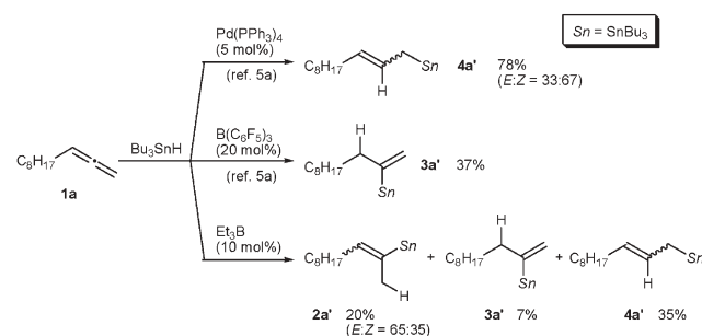
Scheme 1 Hydrostannation of allenes by \text{Bu}_2\text{SnIH} .
