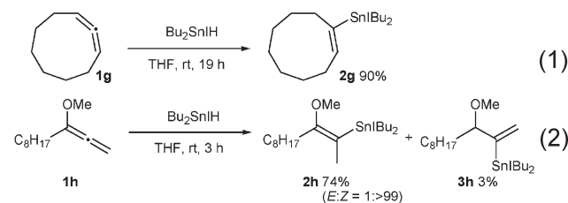
Scheme 2 Hydrostannylation of disubstituted allenes. Reagents : THF (1 mL), allene (1 mmol), \text{Bu}_2\text{SnIH} (1 mmol).
