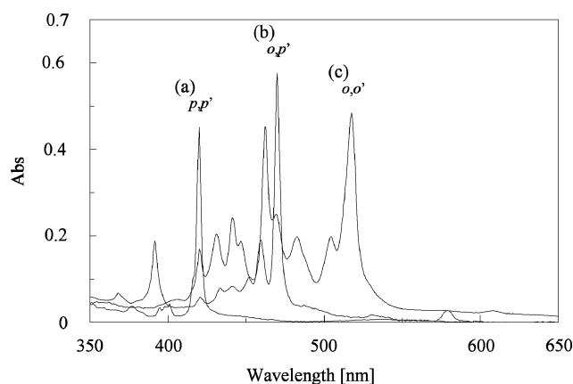
Fig. 6 UV/vis spectrum obtained by irradiation ( \lambda > 390 nm) of (a) 1,2-bis(4-azidophenyl)acetylene ( p,p' -2-N 3 ,N 3 ), (b) 1-(2-azidophenyl)-2-(4-azidophenyl)acetylene ( p,o' -2-N 3 ,N 3 ), and (c) 1,2-bis(2-azidophenyl)acetylene ( o,o' -2-N 3 ,N 3 ) in argon at 13 K.
