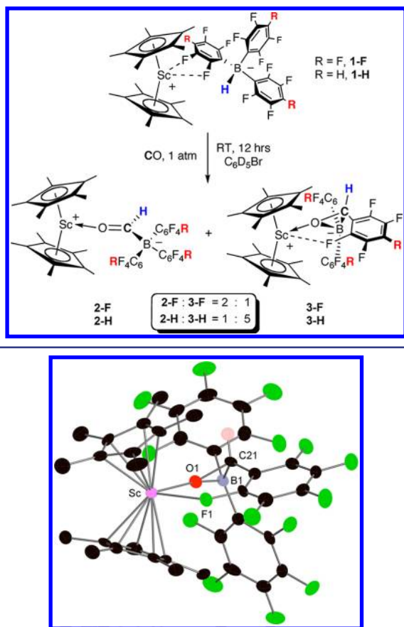
Figure 3. X-ray structure of 3-F (thermal ellipsoids drawn to 50% probability level). All hydrogens except H bonded to C21 are omitted for clarity. Selected bond distances (Å) and angles (deg): Sc–F1, 2.320(4); Sc–O1, 2.187(4); B1–O1, 1.522(8); B1–C21, 1.559(9); O1–C21, 1.478(7). B1–C21–O1, 60.1(4); C21–O1–B1, 62.6(4); O1–B1–C21, 57.3(4).
