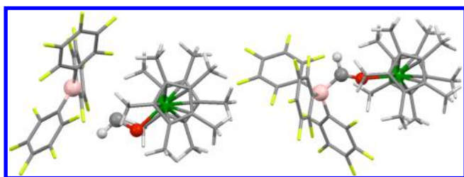
Figure 6. Geometries of TSB (left) and 2-F (right). Sc: green, C gray, B pink, H white. See Figure 4 and Scheme 3 for labeling. Selected geometrical parameters (distances in Å, angles in degrees): TSB: Sc–O 2.11, Sc–C 2.70, B···C 3.1, Sc–O–C 109.0, H–CO 109.4. 2-F: Sc–O 2.09, O–C 1.246 Å, B–C 1.641; Sc–O–C 162.5, H–C–O 114.7, H–C–B 118.0.
