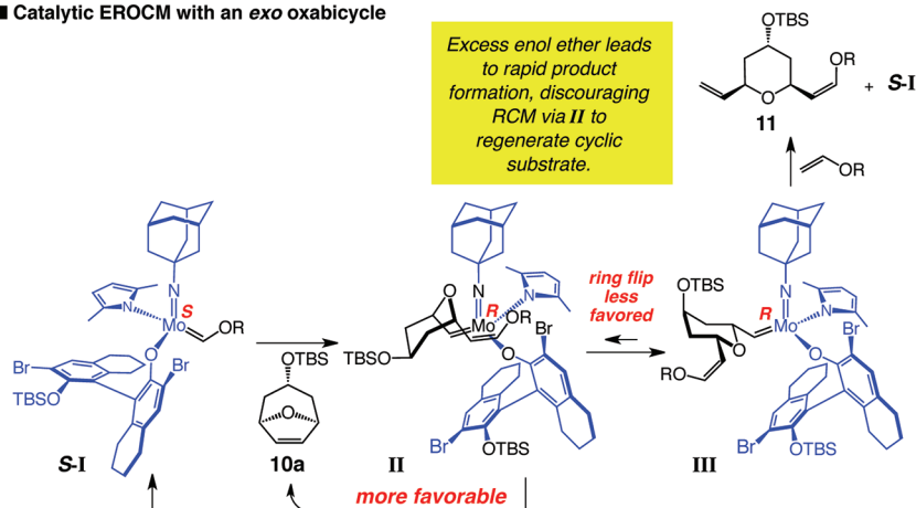
Scheme 3. Relative RCM Rate of ROCM Products as a Function of Stereochemical Identity of the Intermediate Alkylidene
