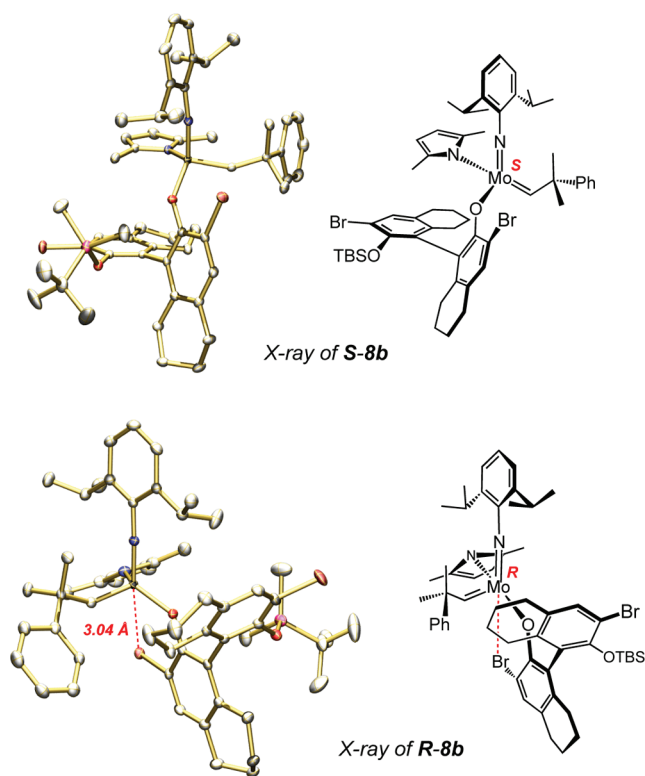
Figure 1. X-ray structures of two diastereomers of a stereogenic-at-Mo monopyrrolide monoaryloxide.
