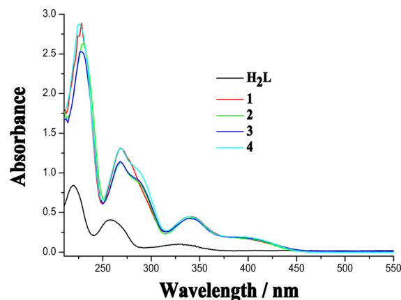
Figure 3. UV–vis absorption spectra of the ligand H 2 L and complexes 1–4 in MeCN solution at 1 \times 10^{-5} M at room temperature.
