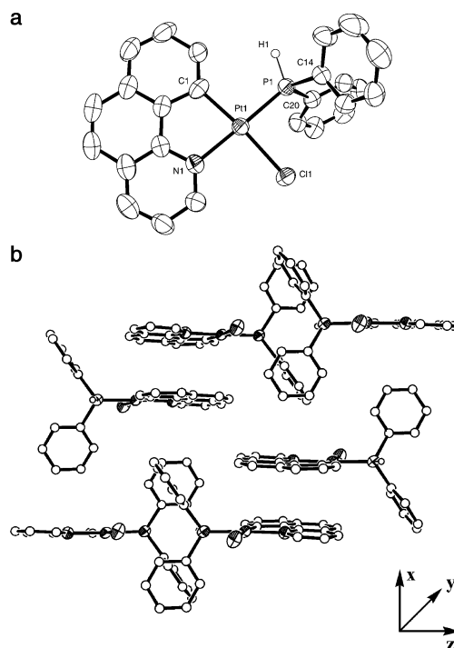
Figure 1. (a) Molecular structure of [Pt(bzq)Cl(PPh 2 H)] 1 . Ellipsoids are drawn at the 50% probability. (b) Packing diagram for 1 .
