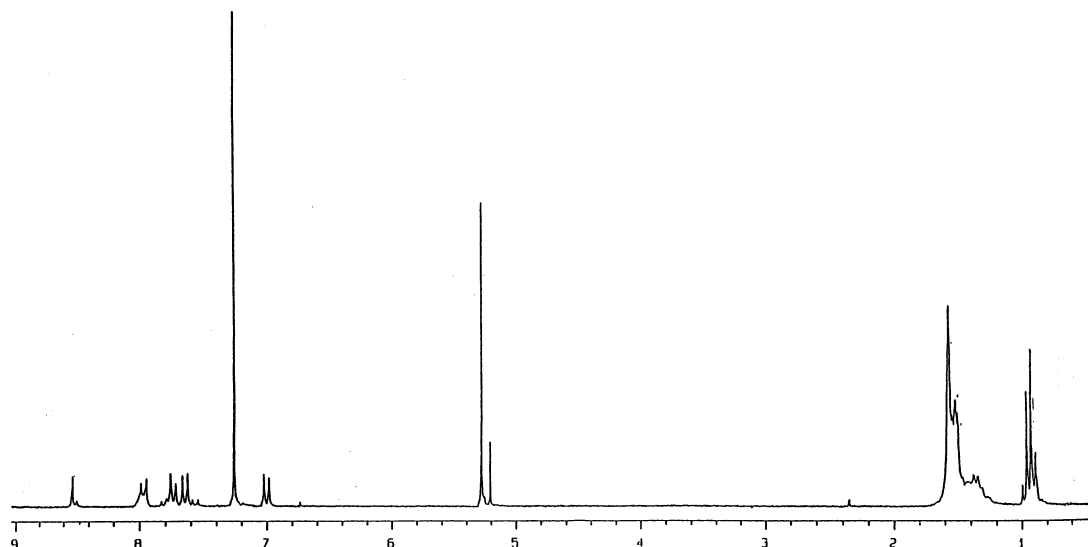
Fig. 1. ^1\text{H} -NMR spectrum of complex 9 .
