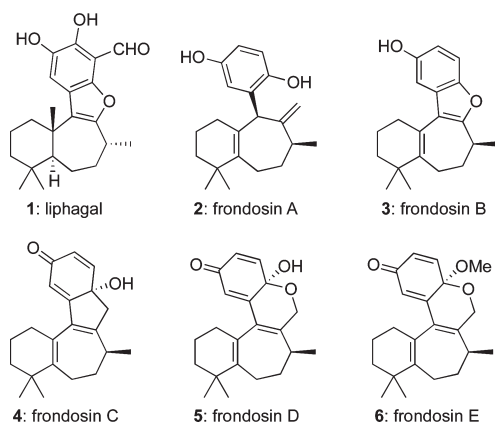
Figure 1. Liphalgal and the frondosins.
