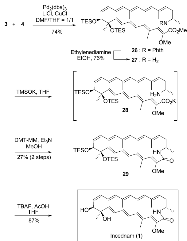
Scheme 3. Total Synthesis of Incednam ( 1 )
