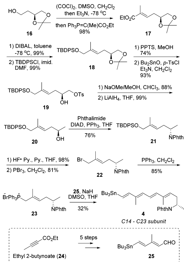
Scheme 2. Synthesis of the C14–C23 Subunit 4
