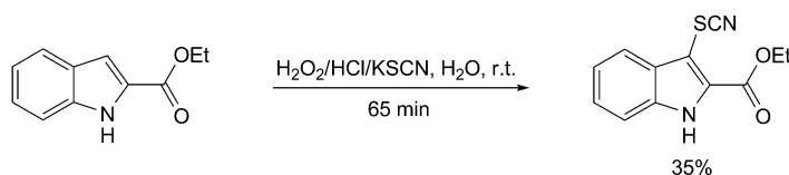
Scheme 2. Thiocyanation of Ethyl 1 H -Indole-2-carboxylate
