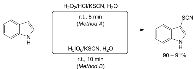
Scheme 1. Conversion of 1 H -Indole to 1 H -Indol-3-yl Thiocyanate
