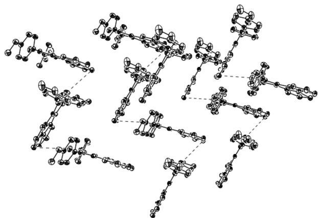
Figure 3. Crystal packing of 5b.
