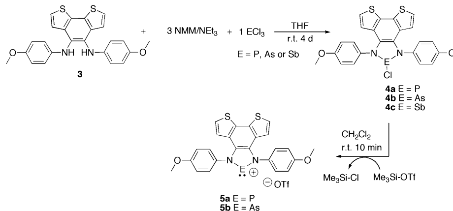
Scheme 2. Synthesis of 4a, 4b, and 4c, and the Subsequent Halide Abstraction Yielding 5a and 5b
