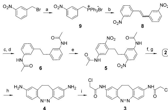
Scheme 1. Synthesis of bridged azobenzene photoswitches 2 and 3 .
