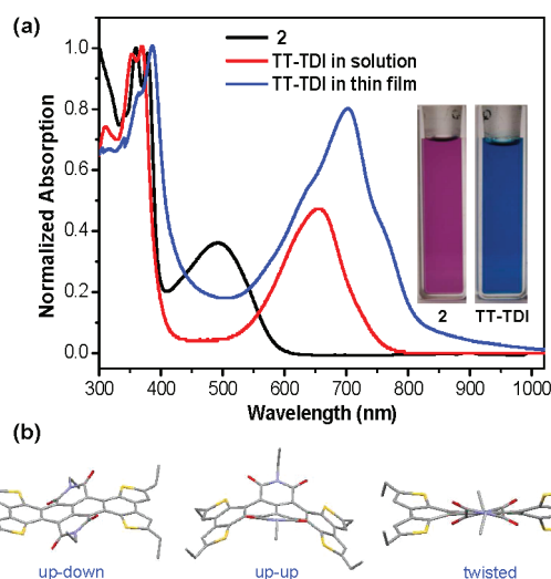
Figure 1. (a) UV-vis absorption spectra of 2 and TT-TDI in chloroform solution ( 1.0 \times 10^{-5} M) and in thin film. Insert: photos for the dilute solution of 2 and TT-TDI in chloroform. (b) Calculated three conformers of TT-TDI .
