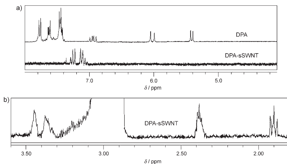
Figure 2. a) ^1\text{H} NMR spectra of DPA (top) and DPA-sSWNTs in [\text{D}_6]\text{DMSO} (bottom, 2.5 \text{ mg mL}^{-1} ), showing the similarities of the peaks in the aromatic region. b) Signals in the aliphatic region of the ^1\text{H} NMR spectrum of DPA-sSWNTs.
