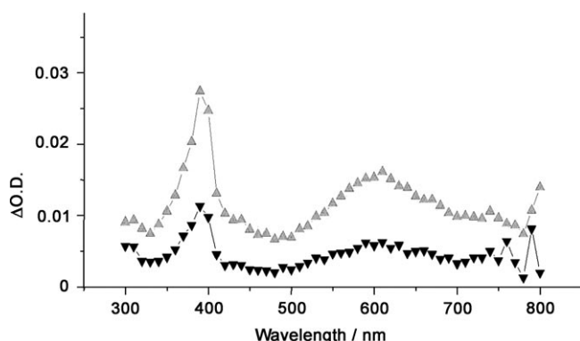
Figure 13. Transient spectra recorded 5.3 (top) and 167 \mu s (bottom) after 355 nm laser excitation of a nitrogen-purged 47 \mu g mL -1 solution of DPA-sSWNTs in DMSO/D 2 O (3:10) upon addition of 100 \mu L of MV^{2+} (0.46 mg mL -1 ). The inset shows the signal decay monitored at 600 nm.
