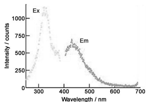
Figure 9. Emission (Em, \lambda_{\text{ex}} = 370 nm) and excitation (Ex, \lambda_{\text{em}} = 430 nm) spectra of a solution of DPA-sSWNTs ( 33.3 \text{ ng mL}^{-1} ) in DMSO/D 2 O (0.1:10).
