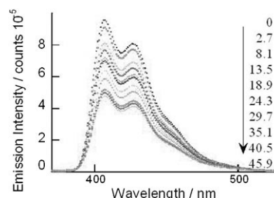
Figure 7. Fluorescence spectra ( \lambda_{\text{ex}} = 370\text{ nm} ) of a nitrogen-purged 70\text{ }\mu\text{M} solution of DPA in acetonitrile ( 1 \times 1\text{ cm}^2 cuvette) upon addition of an increasing concentration of sSWNTs, as indicated (in \text{ng mL}^{-1} ).
