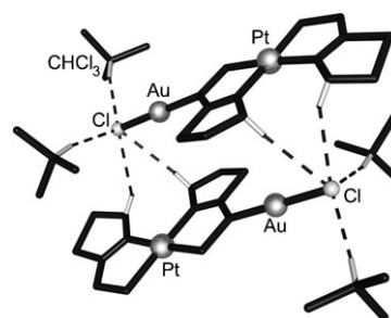
Figure 11. View of the crystal structure of 10·3CHCl 3 , representing a pair of complexes, interconnected by H···Cl contacts and interacting with the solvent through the AuCl moiety. Dashed lines represent H···Cl contacts. White sticks represent the hydrogen atoms involved in these contacts. Protons and phenyls omitted for clarity.
