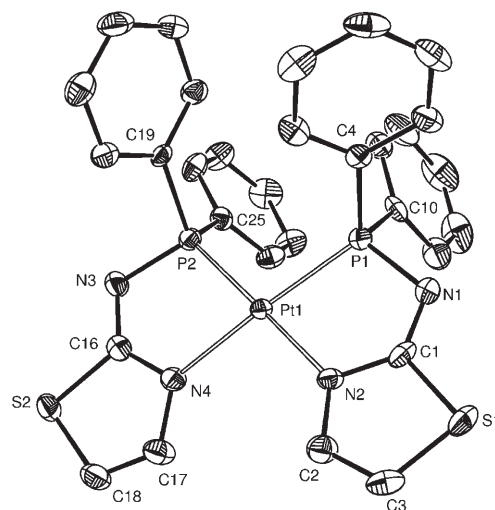
Figure 1. View of the molecular structure of compound cis-6 in cis-6 ·2CH 3 OH·CH 3 CN (Displacement parameters include 50% of the electron density).
