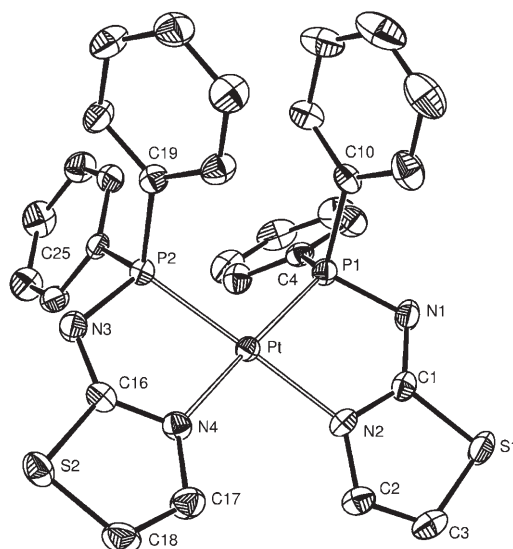
Figure 2. View of the molecular structure of compound cis-7 (Displacement parameters include 50 % of the electron density).
