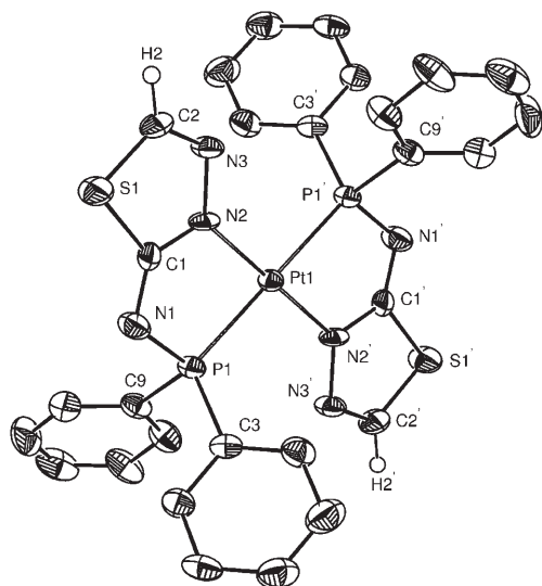
Figure 7. View of the molecular structure of compound trans -9 (displacement parameters include 50% of the electron density). Selected bond distances [Å] and angles [°]: N2–Pt1 2.011(5), P1–Pt1 2.3133(18), N1–P1 1.668(6), C1–N1 1.304(8), C1–N2 1.360(9), C2–N3 1.288(9), C1–S1 1.756(6), C2–S1 1.721(8), N2–Pt1–P1 79.35(16), N2–Pt1–P1 100.65(16). Symmetry operation generating equivalent atoms ('): -x, -y, -z .
