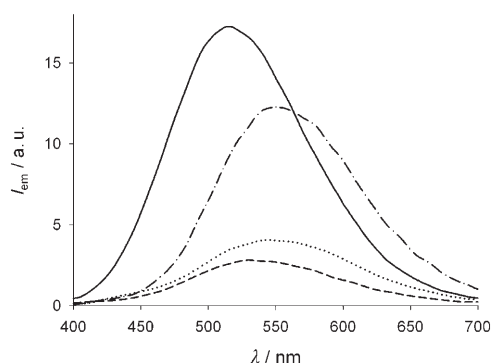
Figure 18. Emission spectra of complex cis-6 crystallized from toluene (dashed line) or exposed to \text{CH}_3\text{OH} (solid line), \text{CH}_3\text{CH}_2\text{OH} (dash-dotted line), or (\text{CH}_3)_2\text{CHOH} (dotted line) at room temperature. \lambda_{\text{ex}} = 313 \text{ nm} . [17]
