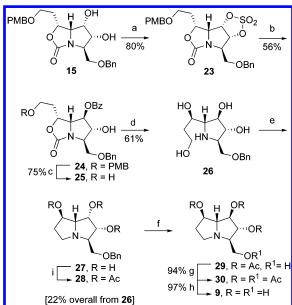
SCHEME 2 a
