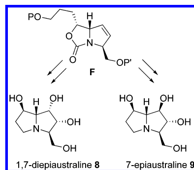
FIGURE 3. Target molecules.
