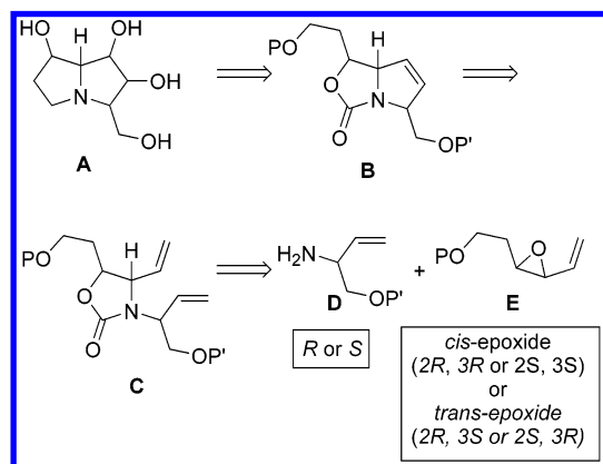
FIGURE 2. Retrosynthetic analysis.
