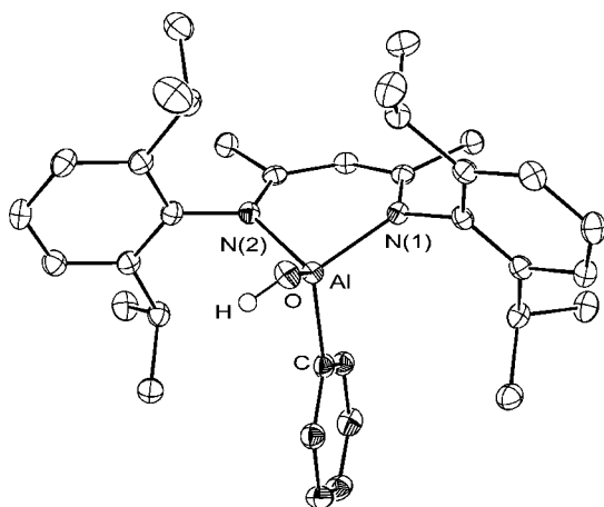
Figure 2. Molecular structure of 11 . Thermal ellipsoids are drawn at the 50% level, and all hydrogen atoms, except that of the OH group, and two THF solvent molecules are omitted for clarity.
