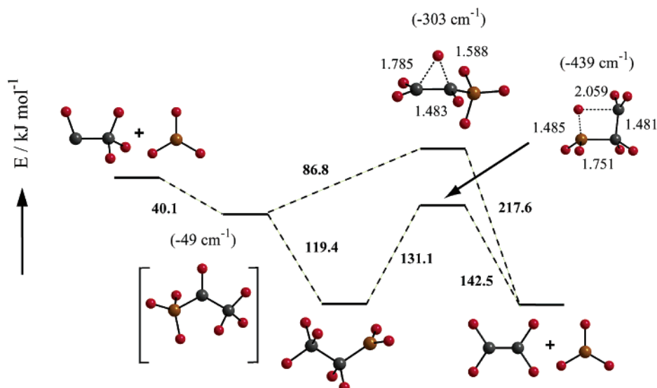
Figure 3. Calculated decomposition of \text{C}_2\text{F}_5\text{BF}_2 (energy and geometry, B3LYP/6-311+G(d); wavenumbers and ZPC, B3LYP/6-311G(d)).
