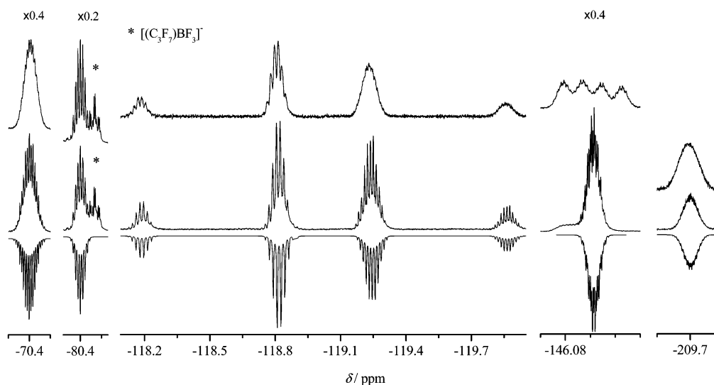
Figure 13. Simulated ^{19}\text{F}\{^{11}\text{B}\} NMR (bottom), ^{19}\text{F}\{^{11}\text{B}\} NMR (middle), and ^{19}\text{F} NMR spectrum (top) of [(\text{C}_2\text{F}_5)(\text{CF}_3)\text{FCBF}_3]^- .
