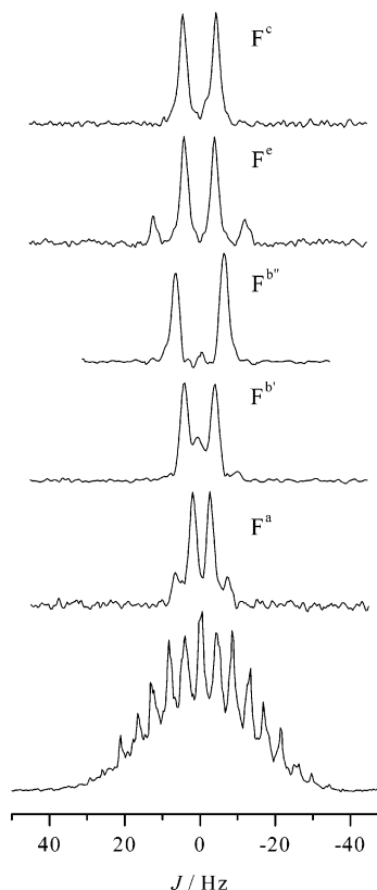
Figure 8. ^{19}\text{F}\{^{11}\text{B}\} NMR spectrum of [(\text{CF}_3)_3\text{CF}^{\text{b}'}\text{F}^{\text{b}''}](\text{CF}_3)_3\text{F}^{\text{c}}\text{CF}^{\text{b}}\text{F}_3]^- (bottom) and F2 projections, ^nJ(^{19}\text{F}, ^{19}\text{F}) , obtained by SERF experiments.
