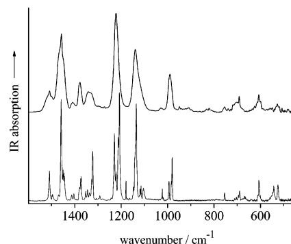
Figure 1. Gas phase and solid state IR (Ar matrix) spectra of \text{C}_2\text{F}_5\text{BF}_2 .
