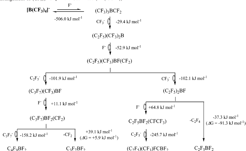
Scheme 2. Rearrangement of (\text{CF}_3)_3\text{BCF}_2 in the Gas Phase ( \Delta E(298 \text{ K})^a )
