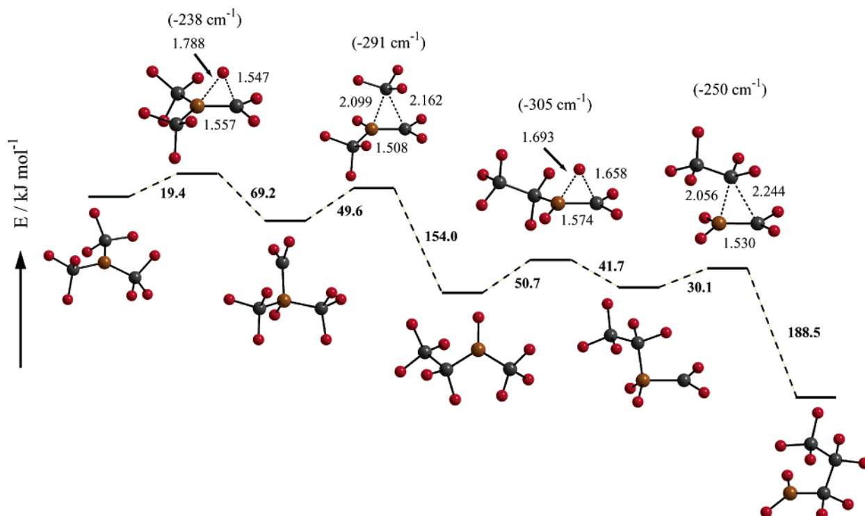
Figure 4. Calculated reaction profile for the isomerization of (\text{CF}_3)_3\text{B} to \text{C}_3\text{F}_7\text{BF}_2 (energy and geometry, B3LYP/6-311+G(d); wavenumbers and ZPC, B3LYP/6-311G(d)).
