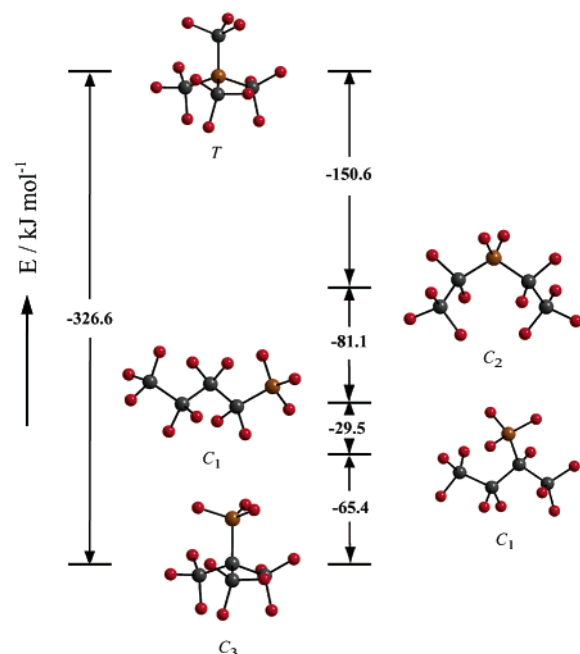
Figure 7. Comparison of the relative stabilities ( \Delta H ) of some [\text{C}_4\text{BF}_{12}]^- anions (energy and geometry, B3LYP/6-311+G(d); ZPC and thermal corrections, B3LYP/6-311G(d)).
