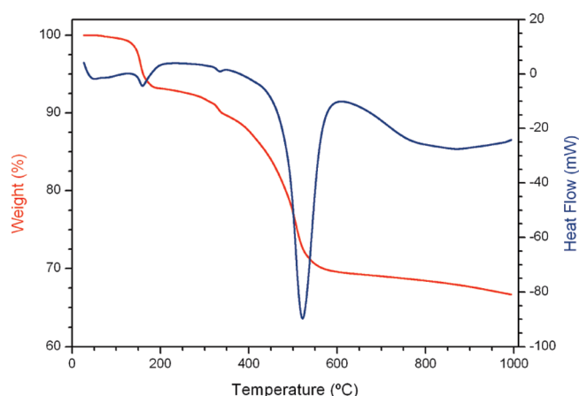
Figure 5. TGA (red) and DTA (blue) curves for the degradation of 14 \cdot C_7H_8 under Ar flow at a heating rate of 10\text{ }^{\circ}C/\text{min} .
