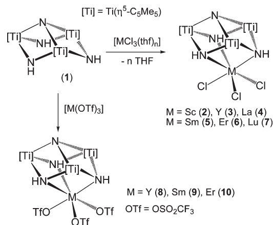
Scheme 1. Reactions of 1 with [\text{MCl}_3(\text{thf})_n] or [\text{M}(\text{OTf})_3]
