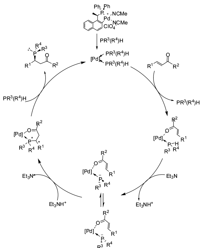
Scheme 2. Proposed Catalytic Cycle
