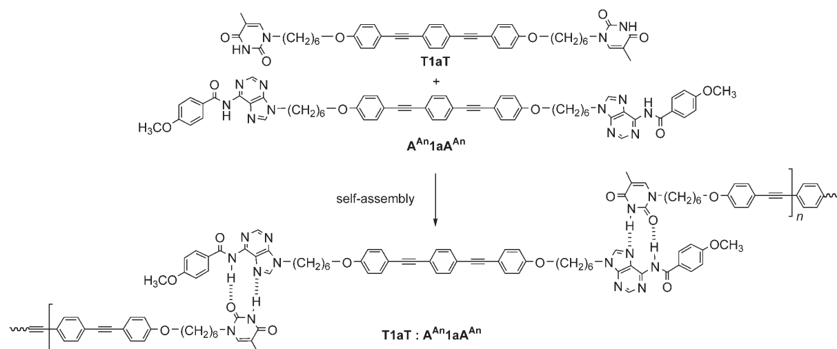
Scheme 2. Proposed nucleobase-induced, self-assembled fluorescent polymer ( T1aT:A An 1aA An ).
