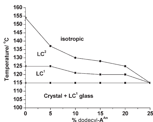
Figure 10. Phase diagram depicting the effects of monofunctional dodecyl- A An on the liquid-crystalline phase of the T1aT:A An 1aA An mixture.
