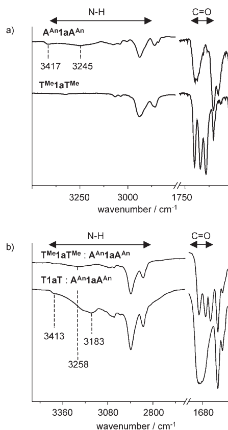
Figure 11. IR spectra of the NH stretching region and the carbonyl region of a) \text{T}^{\text{Me}}\text{1aT}^{\text{Me}} vs \text{A}^{\text{An}}\text{1aA}^{\text{An}} and b) \text{T1aT}:\text{A}^{\text{An}}\text{1aA}^{\text{An}} vs \text{T}^{\text{Me}}\text{1aT}^{\text{Me}}:\text{A}^{\text{An}}\text{1aA}^{\text{An}} mixtures.
