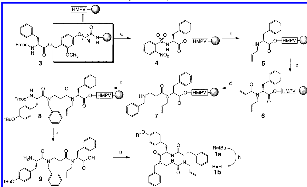
Scheme 2. Synthesis of a Representative Mimetic a
