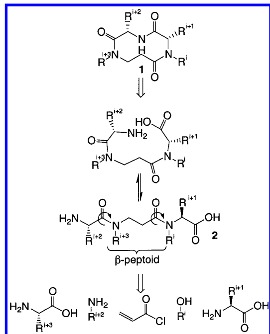
Scheme 1. Retrosynthesis of \beta -Turn Mimetics with General Structure 1
