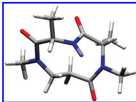
Figure 3. Global minimum of the \alpha_2\beta -tripeptide backbone. The calculated torsion angles were \Phi^{i+1} = 59^\circ , \psi^{i+1} = 44^\circ , \Phi^{i+2} = 66^\circ , \psi^{i+2} = 30^\circ .
