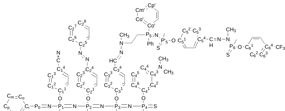
Scheme 4. Numbering scheme used for the NMR assignments
