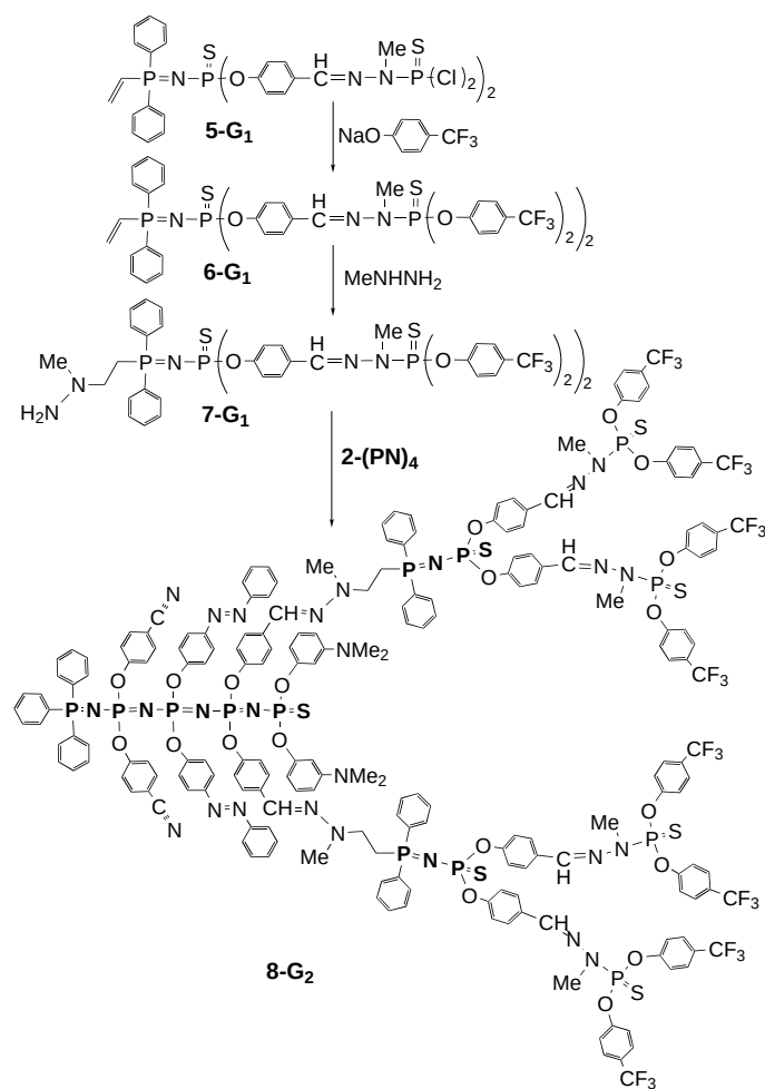
Scheme 3. Regioselective grafting of two dendrons on the oligophosphazene 2-(PN) 4 .
