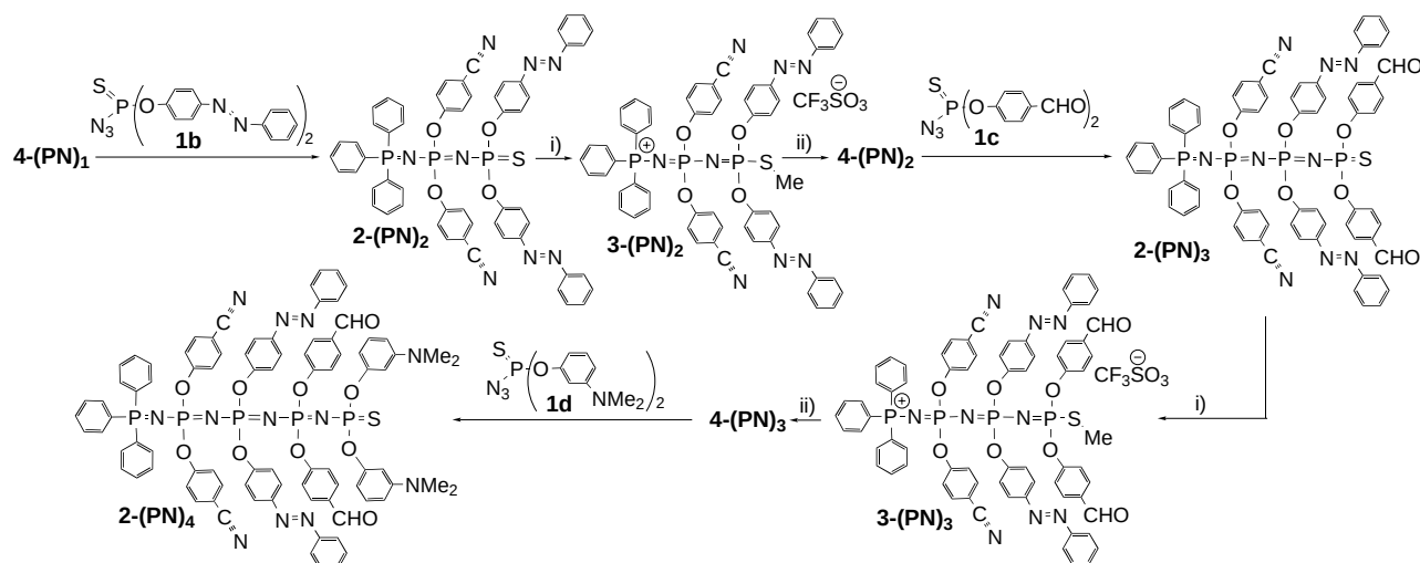
Scheme 2. Repetitive multistep synthesis of the tetraphosphazene 2-(PN) 4 . i) CF 3 SO 3 Me; ii) P(NMe 2 ) 3 , –[MeSP(NMe 2 ) 3 ][CF 3 SO 3 ].
